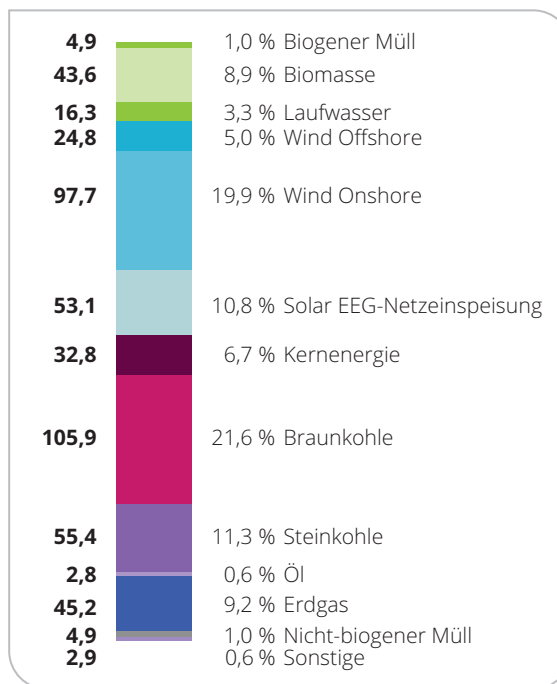
Abb. 92, Quelle: https://www.energy-charts.info/charts/energy_pie/chart.html?l=de&c=DE&interval=year&year=2022
